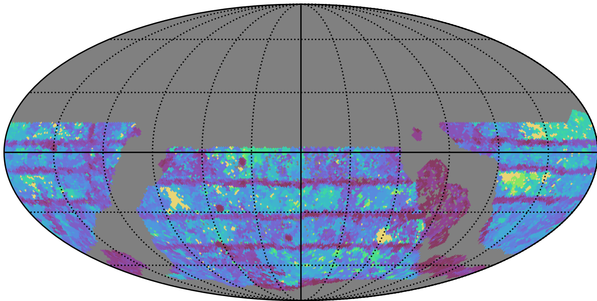
ddf_acor_sf10_lsf30_lsr10_v3.4_10yrs WFD r band: Max Inter-Night Gap
