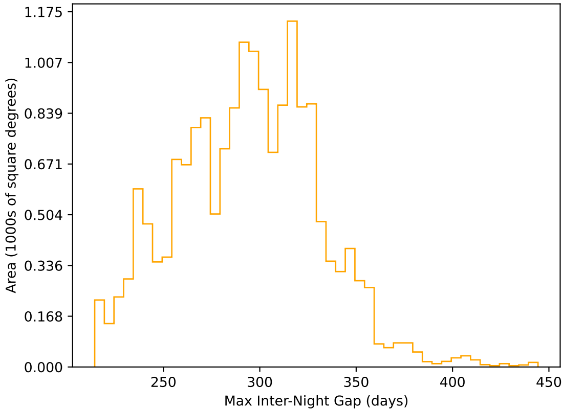
ddf_acor_sf10_lsf30_lsr10_v3.4_10yrs WFD r band: Max Inter-Night Gap
