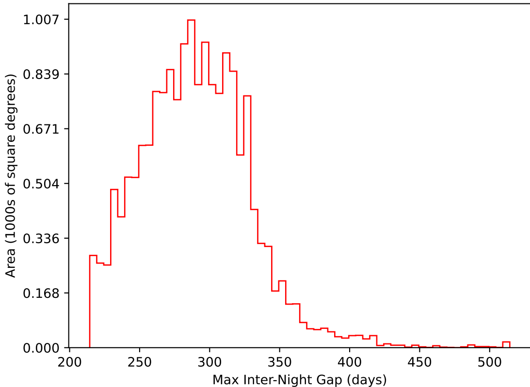
ddf_acor_sf10_ls30_lsr10_v3.4_10yrs WFD i band: Max Inter-Night Gap
