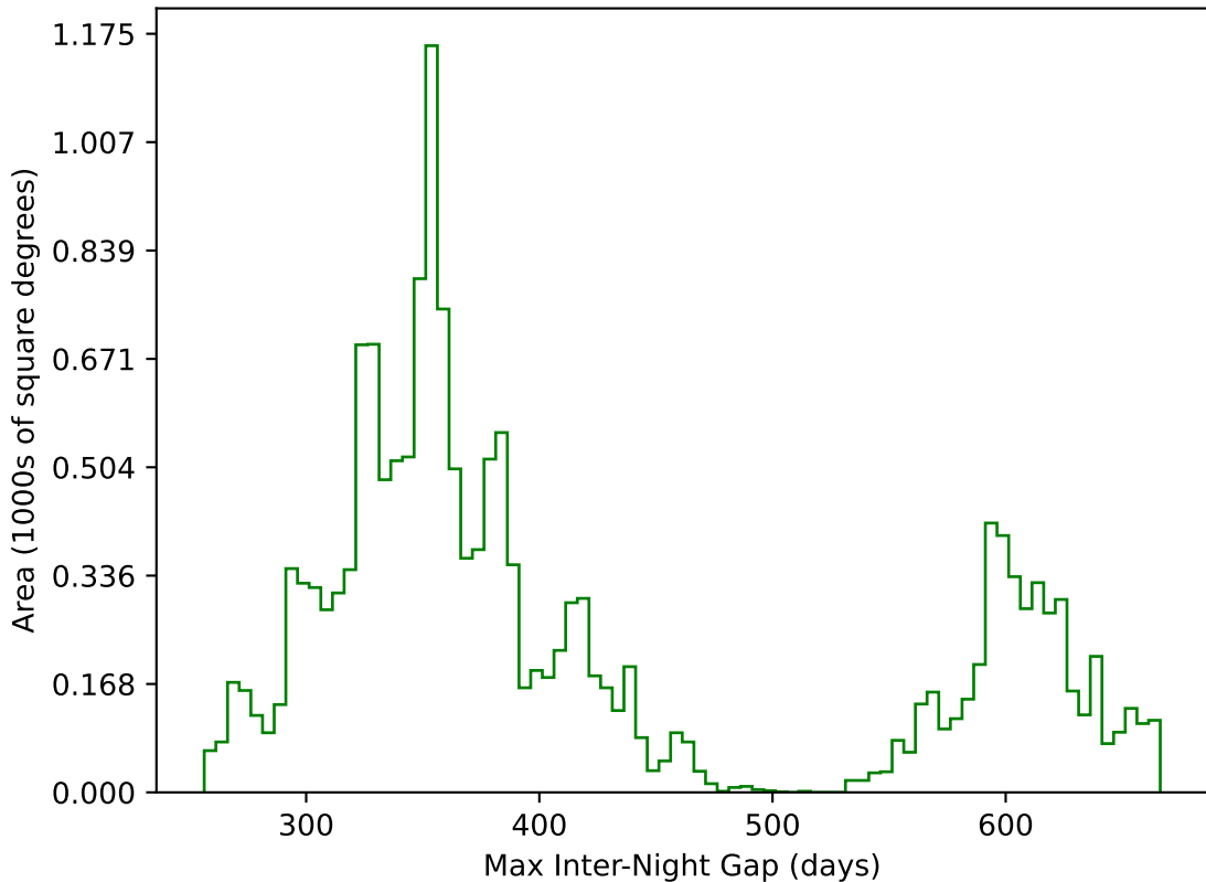
ddf_acor_sf10_lsf30_lsr10_v3.4_10yrs WFD g band: Max Inter-Night Gap
