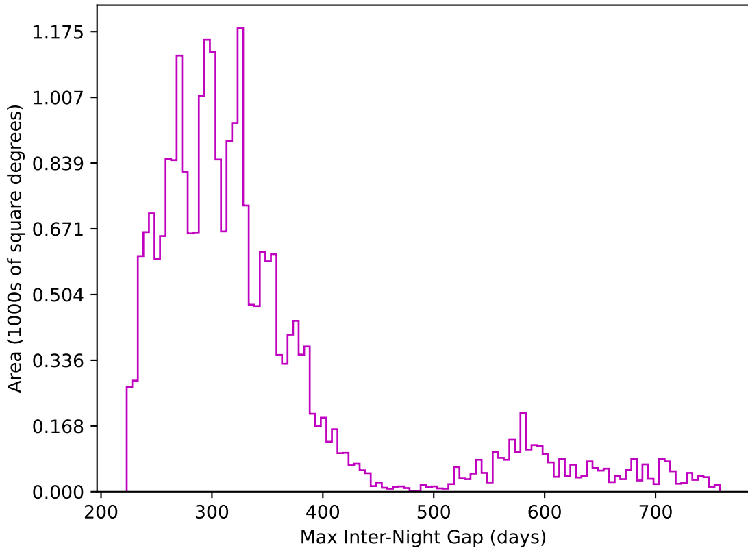
ddf_acor_sf10_lsf30_lsr10_v3.4_10yrs All sky z band: Max Inter-Night Gap
