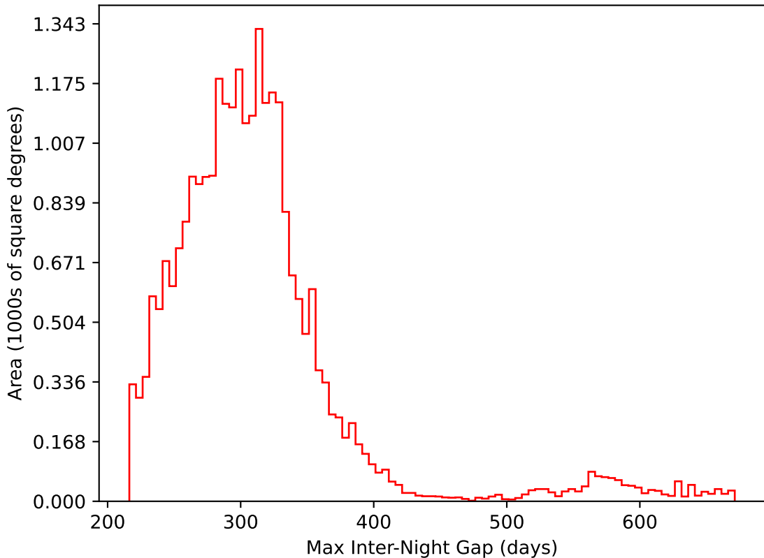
ddf_acor_sf10_lsf30_lsr10_v3.4_10yrs All sky i band: Max Inter-Night Gap
