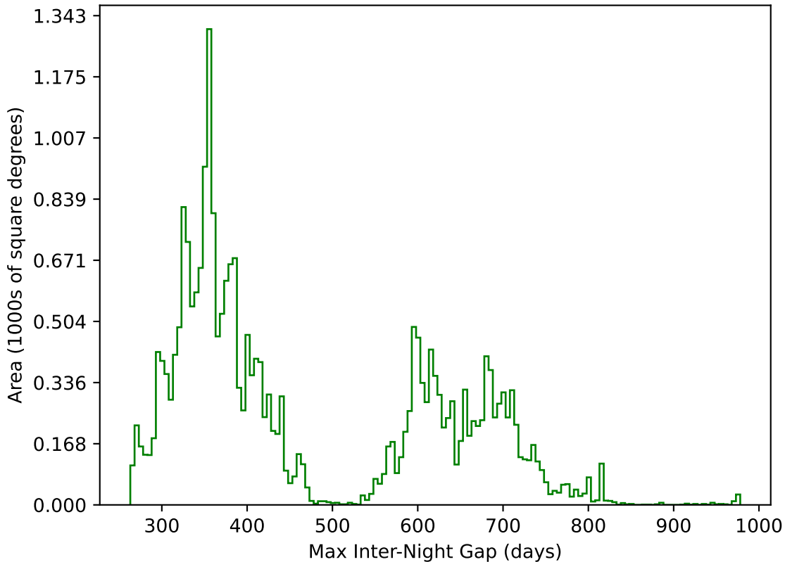
ddf_acor_sf10_lsf30_lsr10_v3.4_10yrs All sky g band: Max Inter-Night Gap
