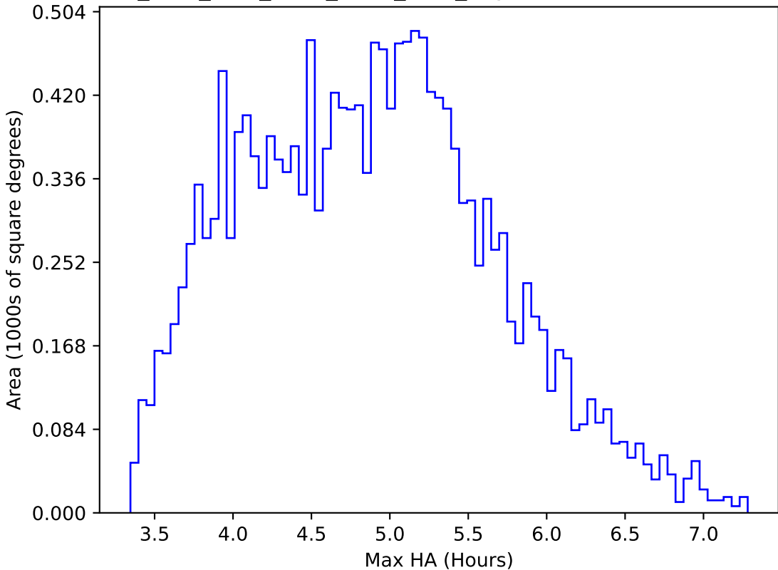
ddf_acor_sf10_lsf30_lsr10_v3.4_10yrs WFD z band: Max HA
