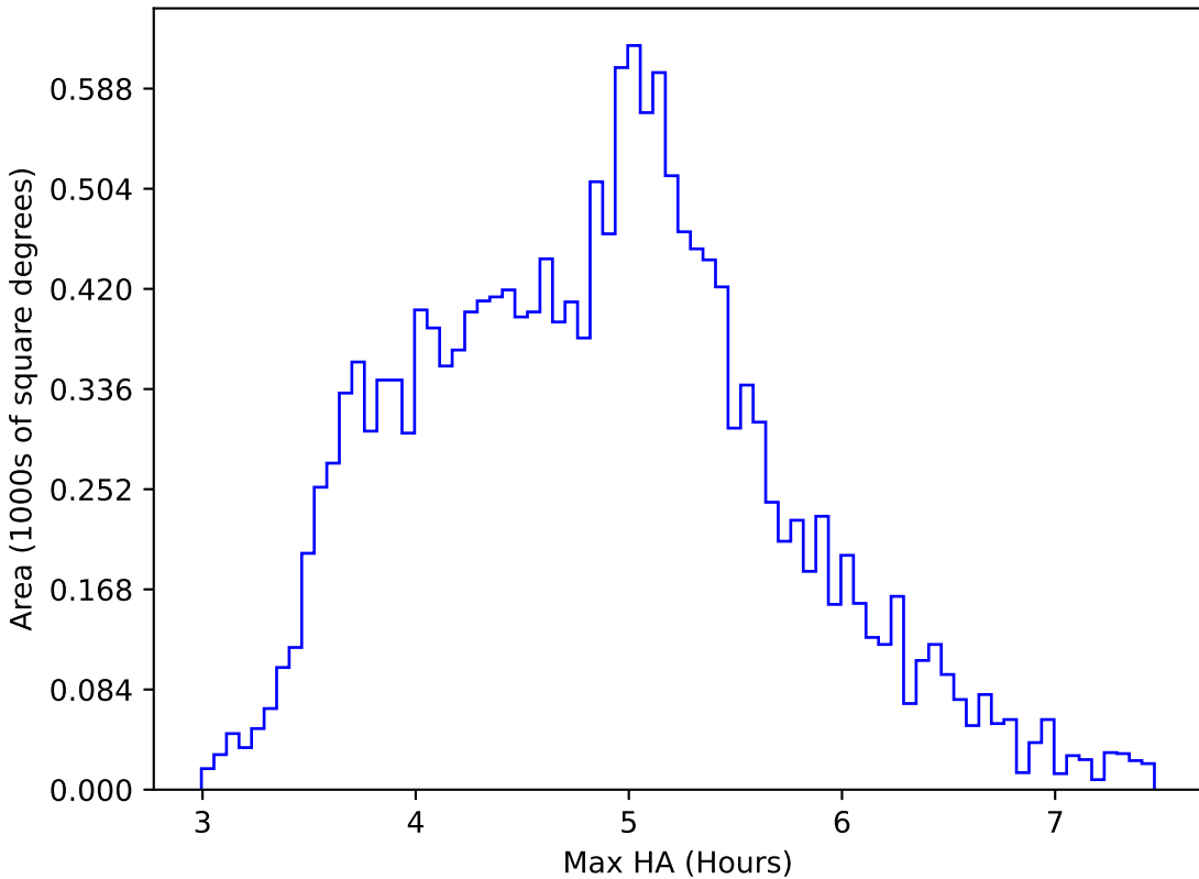
ddf_acor_sf10_lsf30_lsr10_v3.4_10yrs WFD i band: Max HA
