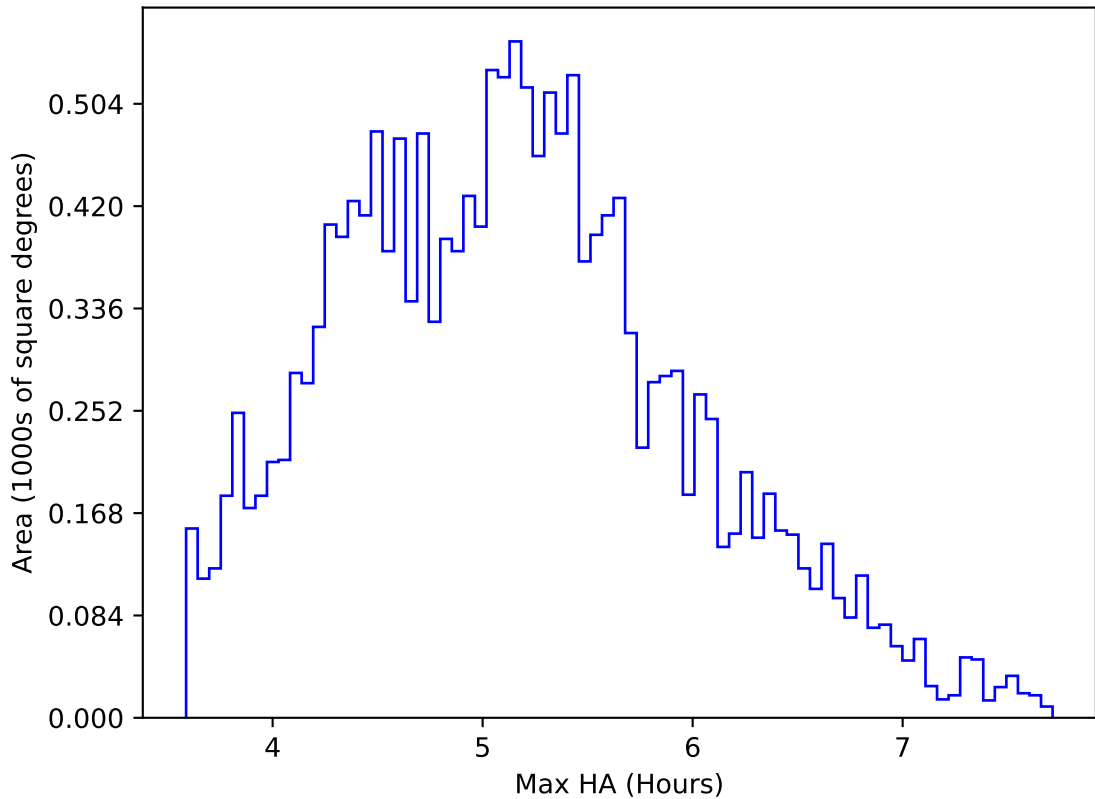
ddf_acor_sf10_lsf30_lsr10_v3.4_10yrs WFD all bands: Max HA
