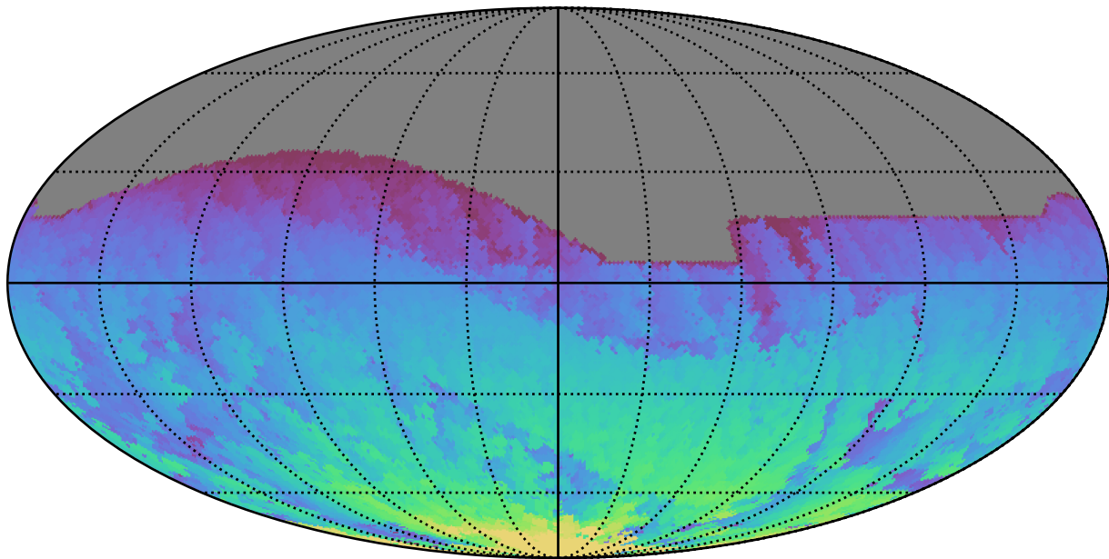
ddf_acor_sf10_lsf30_lsr10_v3.4_10yrs All sky z band: Max HA
