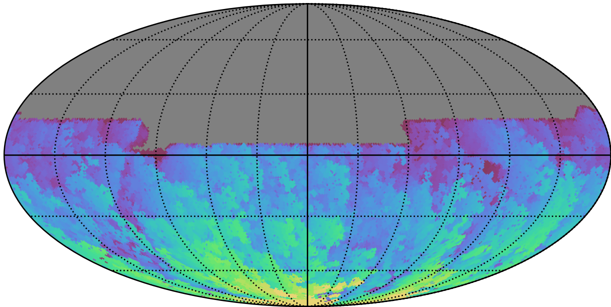
ddf_acor_sf10_lsf30_lsr10_v3.4_10yrs All sky u band: Max HA
