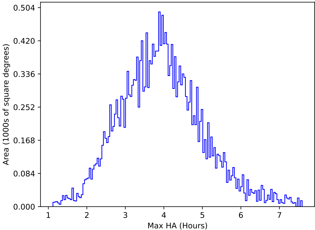
ddf_acor_sf10_lsf30_lsr10_v3.4_10yrs All sky u band: Max HA
