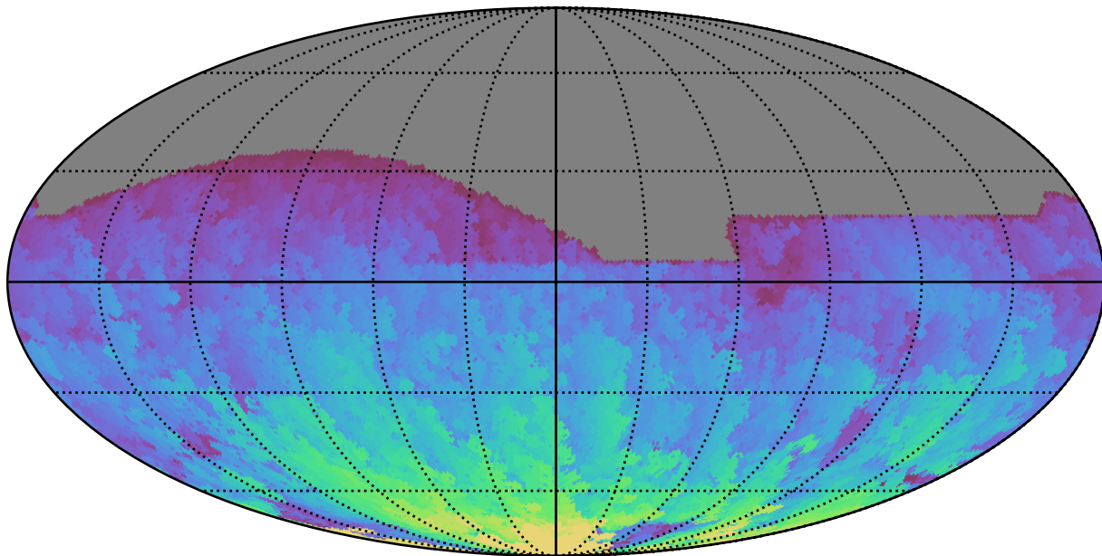
ddf_acor_sf10_lsf30_lsr10_v3.4_10yrs All sky r band: Max HA
