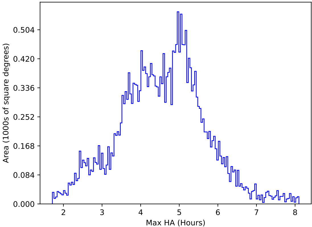
ddf_acor_sf10_lsf30_lsr10_v3.4_10yrs All sky i band: Max HA
