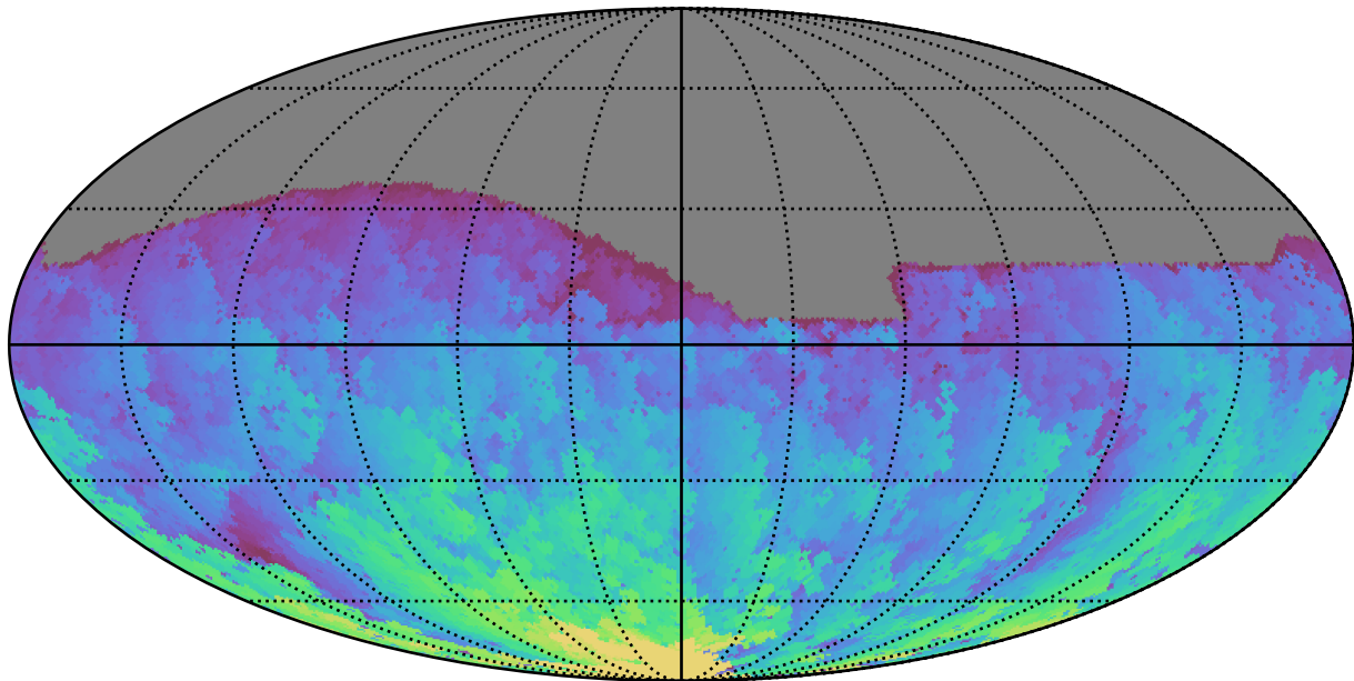
ddf_acor_sf10_lsf30_lsr10_v3.4_10yrs All sky g band: Max HA
