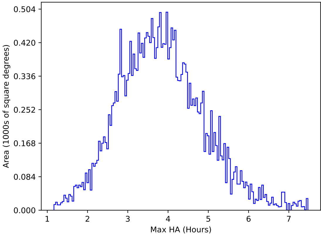
ddf_acor_sf10_lsf30_lsr10_v3.4_10yrs All sky g band: Max HA
