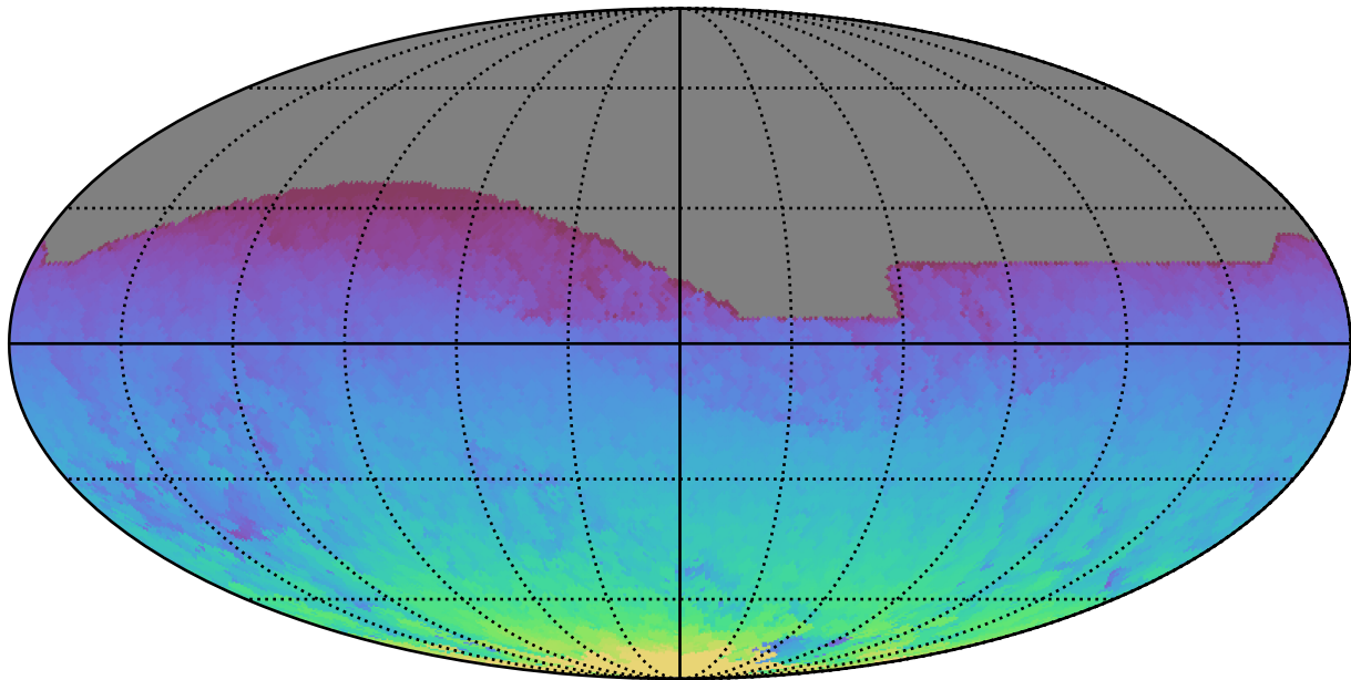
ddf_acor_sf10_lsf30_lsr10_v3.4_10yrs All sky all bands: Max HA
