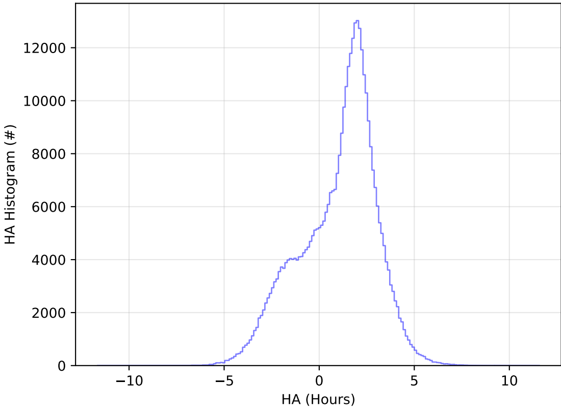
ddf_acor_sf10_ls30_lsr10_v3.4_10yrs WFD y band: HA Histogram
