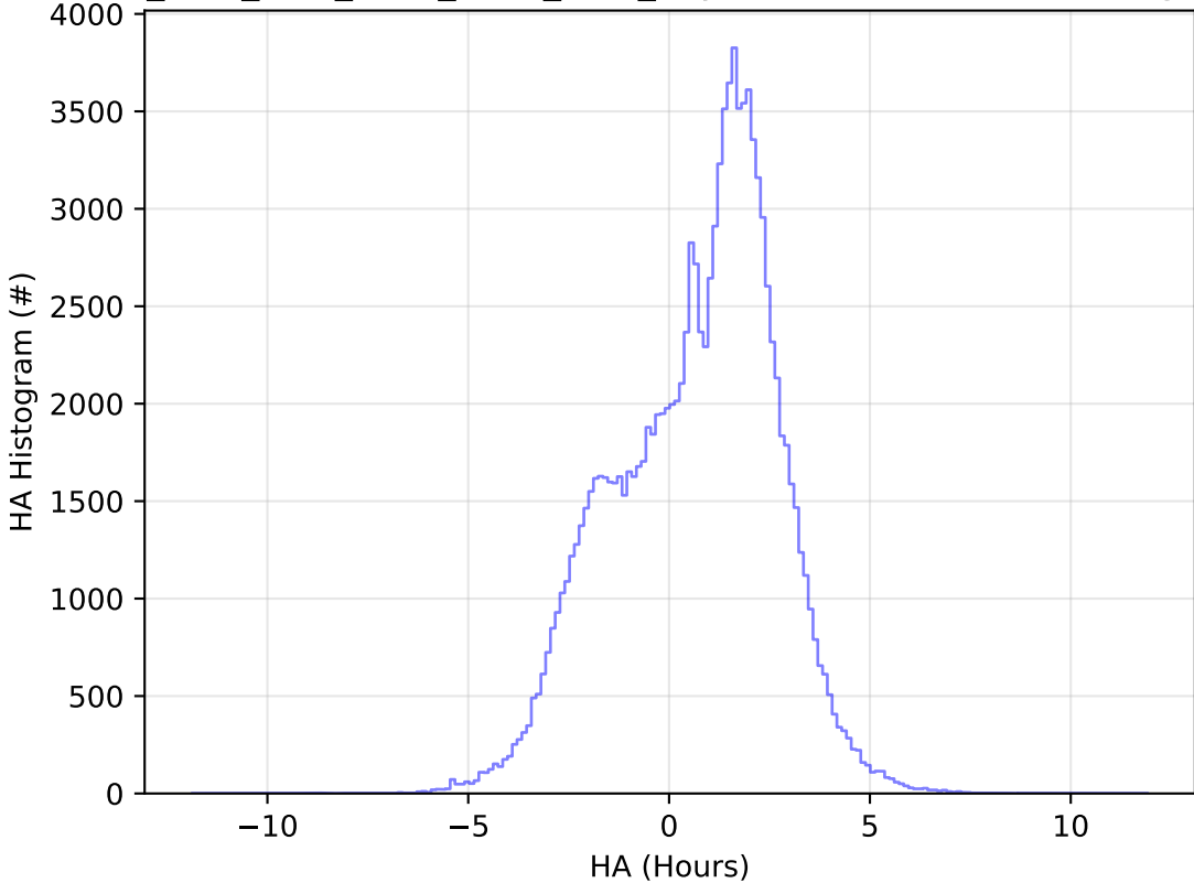
ddf_acor_sf10_lsf30_lsr10_v3.4_10yrs WFD u band: HA Histogram
