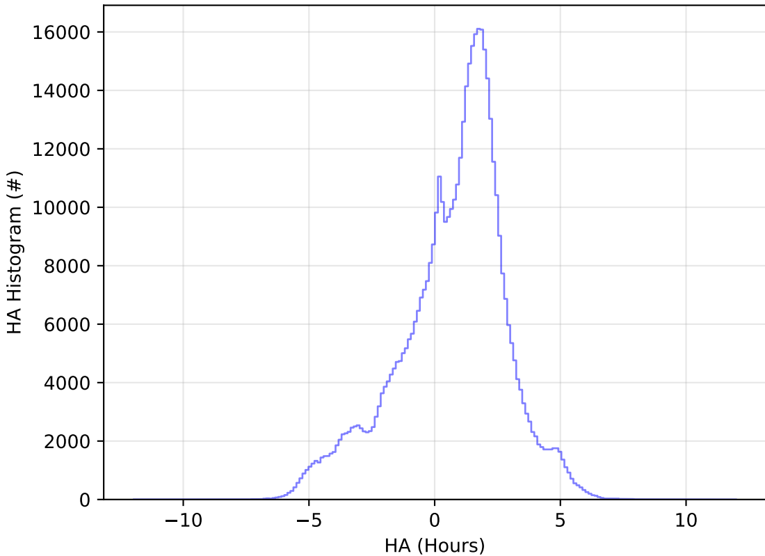
ddf_acor_sf10_lsf30_lsr10_v3.4_10yrs WFD i band: HA Histogram
