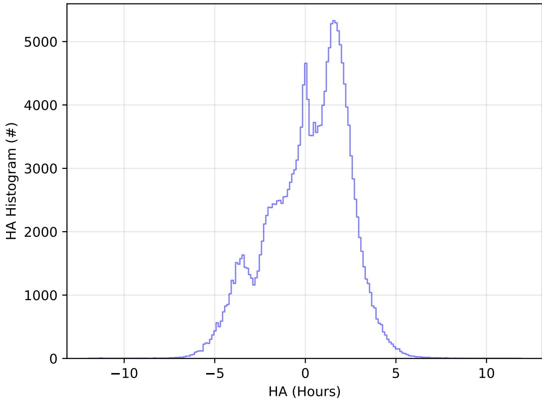
ddf_acor_sf10_lsf30_lsr10_v3.4_10yrs WFD g band: HA Histogram
