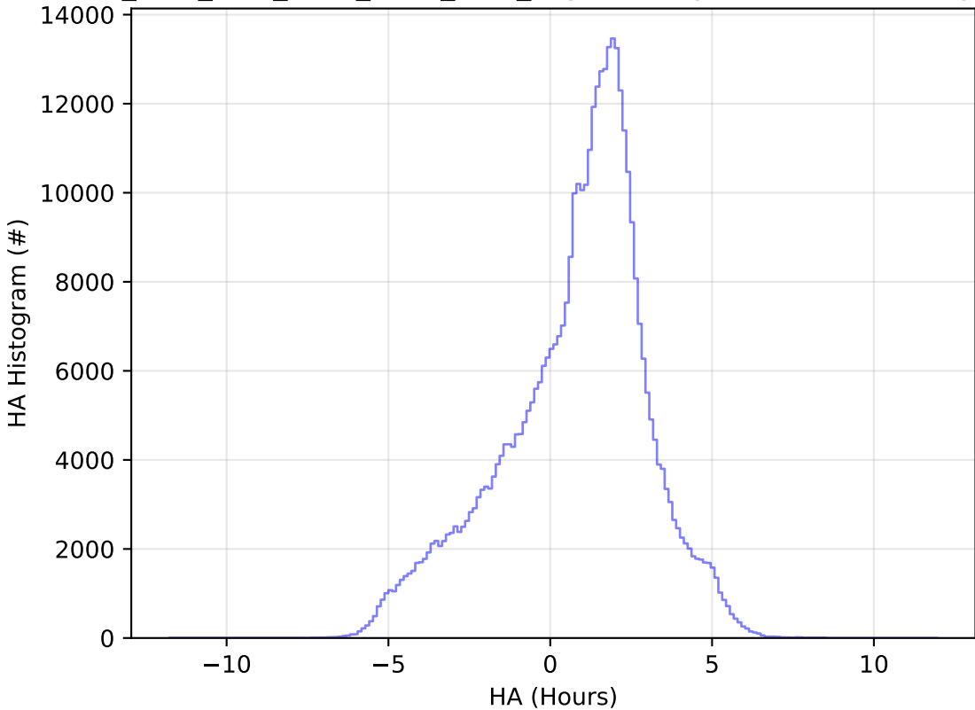
ddf_acor_sf10_lsf30_lsr10_v3.4_10yrs All sky z band: HA Histogram
