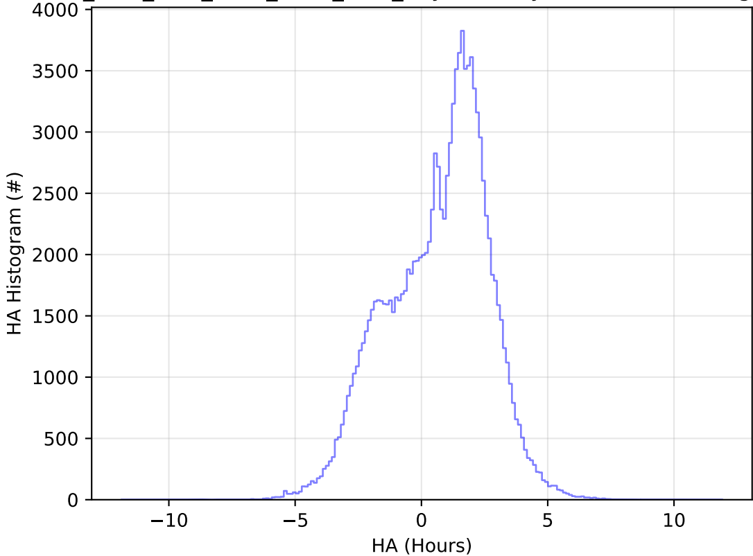
ddf_acor_sf10_lsf30_lsr10_v3.4_10yrs All sky u band: HA Histogram
