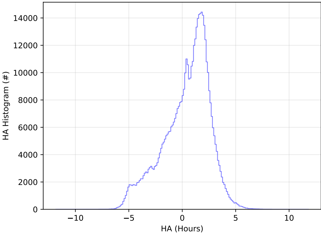
ddf_acor_sf10_lsf30_lsr10_v3.4_10yrs All sky r band: HA Histogram
