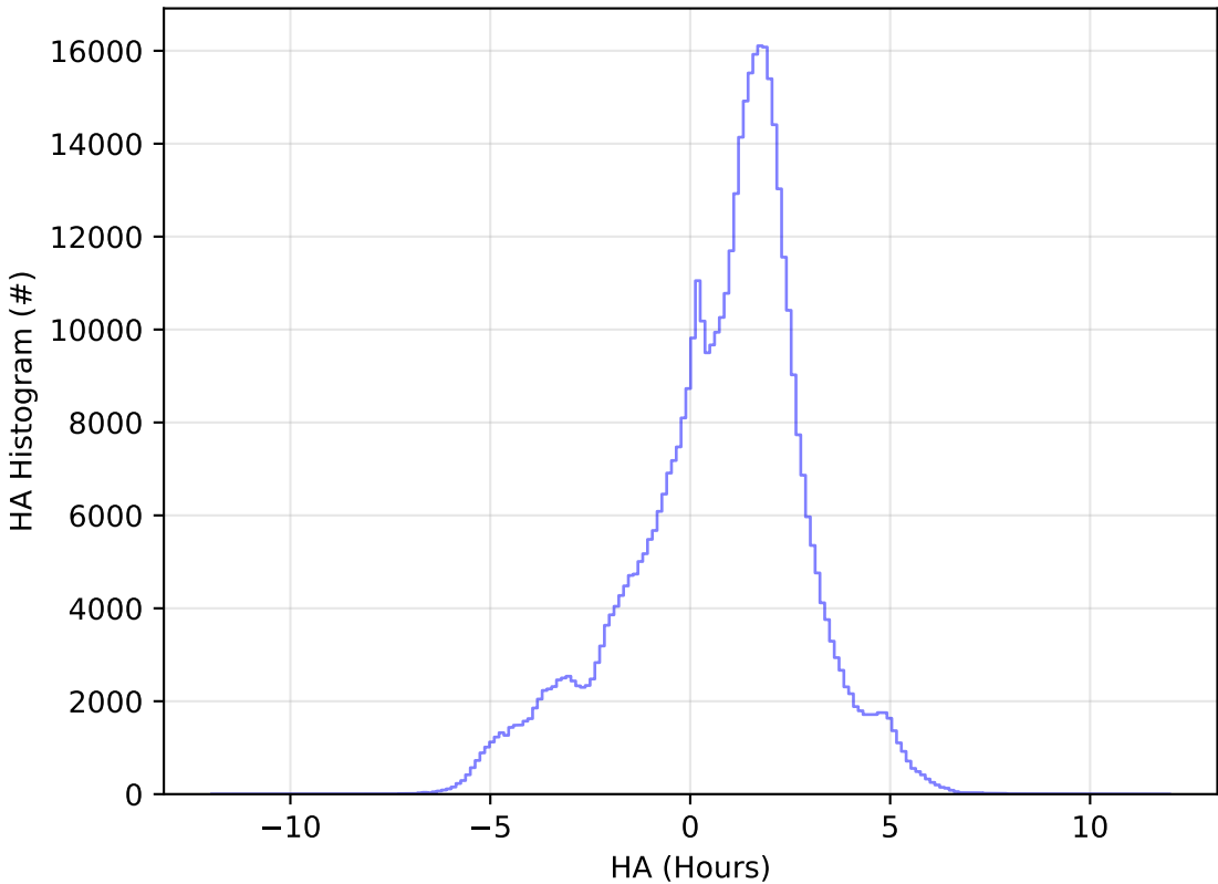
ddf_acor_sf10_lsf30_lsr10_v3.4_10yrs All sky i band: HA Histogram
