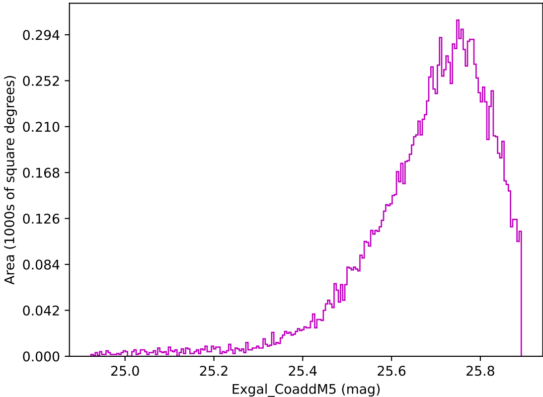
ddf_acor_sf10_lsf30_lsr10_v3.4_10yrs WFD z band: Exgal_CoaddM5
