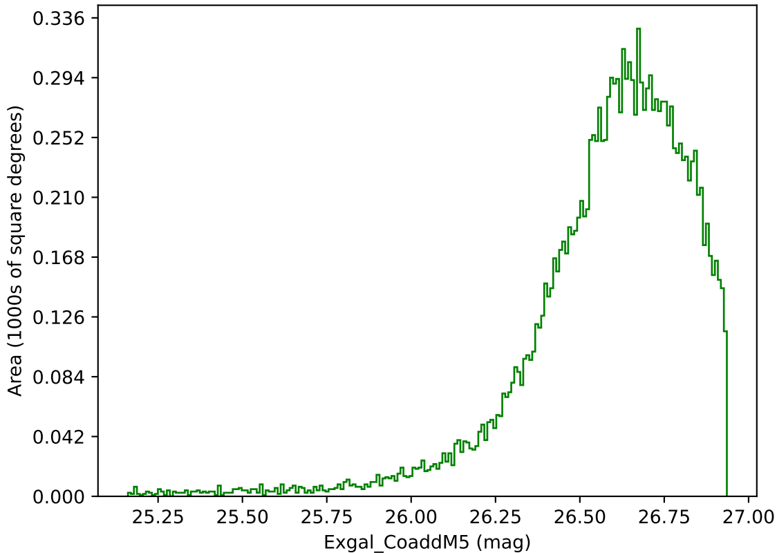
ddf_acor_sf10_lsf30_lsr10_v3.4_10yrs WFD g band: Exgal_CoaddM5
