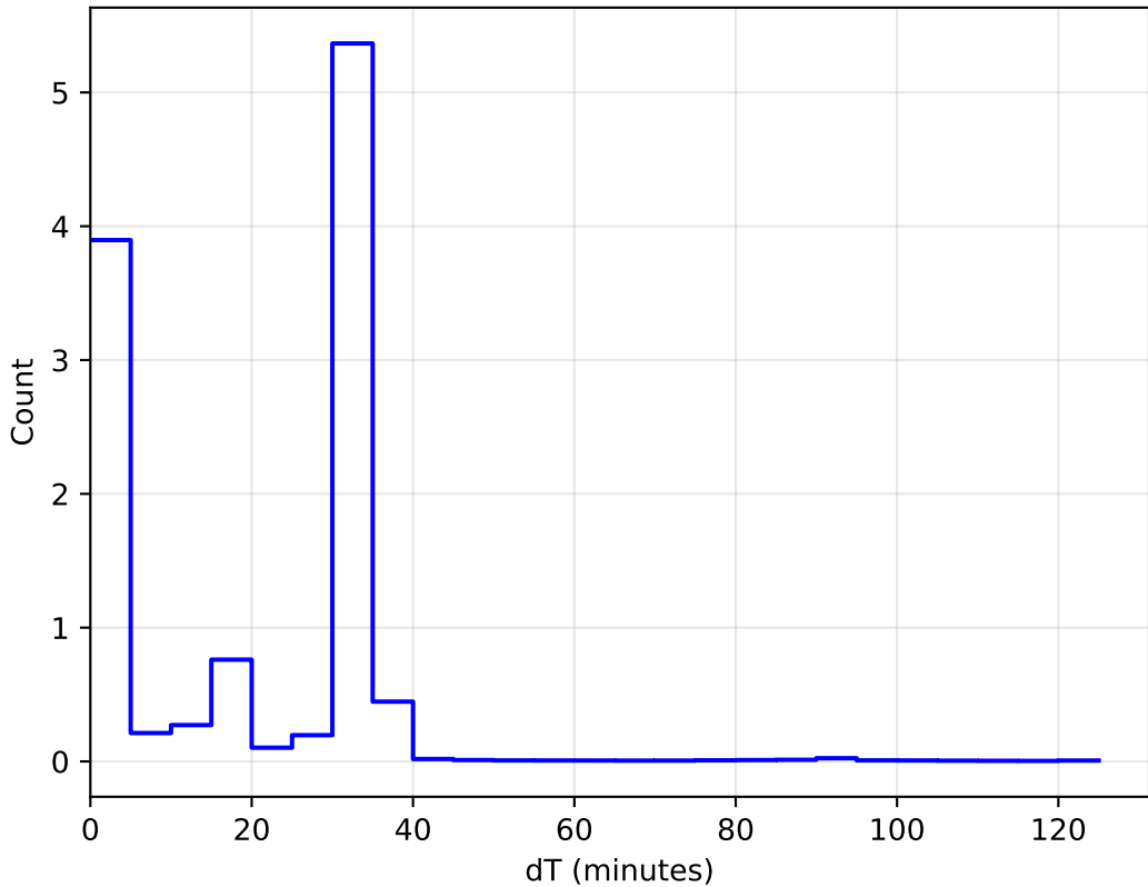
ddf_acor_sf10_lsf30_lsr10_v3.4_10yrs WFD: DeltaT Histogram 1e6
