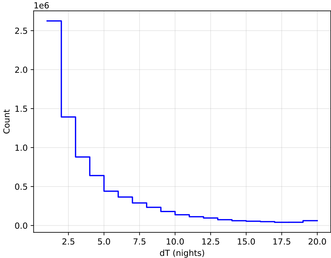
ddf_acor_sf10_lsf30_lsr10_v3.4_10yrs WFD all bands: DeltaNight Histogram
