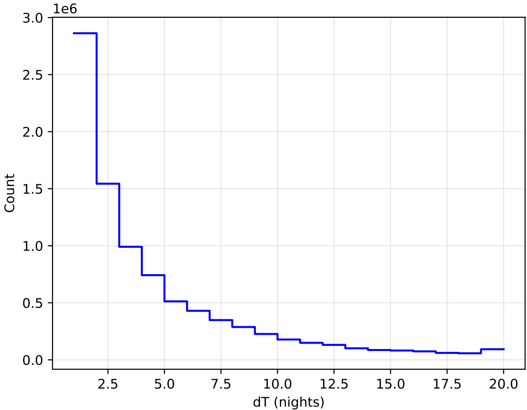
ddf_acor_sf10_lsf30_lsr10_v3.4_10yrs All sky all bands: DeltaNight Histogram
