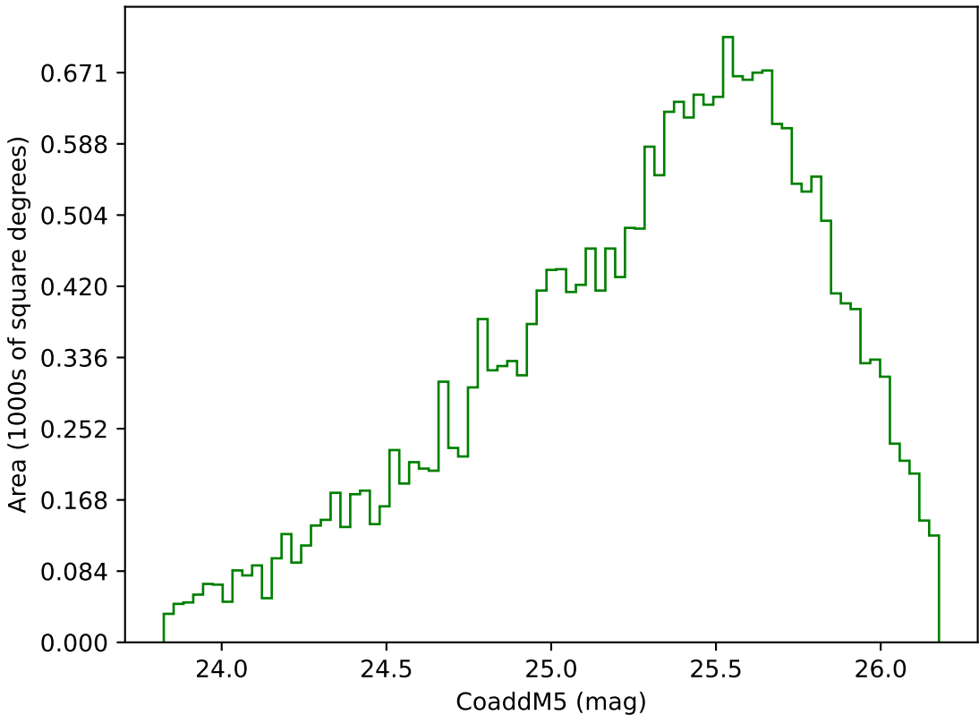
ddf_acor_sf10_lsf30_lsr10_v3.4_10yrs Yr 3-4 g band: CoaddM5
