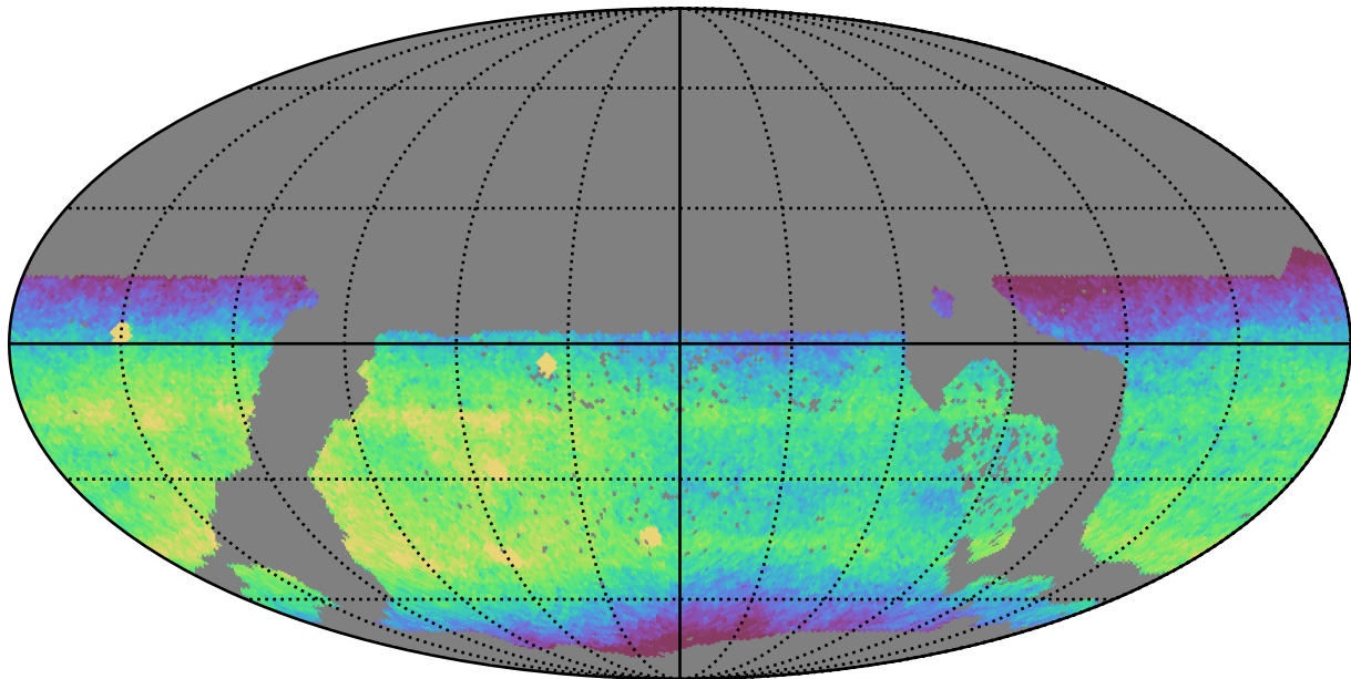
ddf_acor_sf10_lsf30_lsr10_v3.4_10yrs WFD i band: CoaddM5
