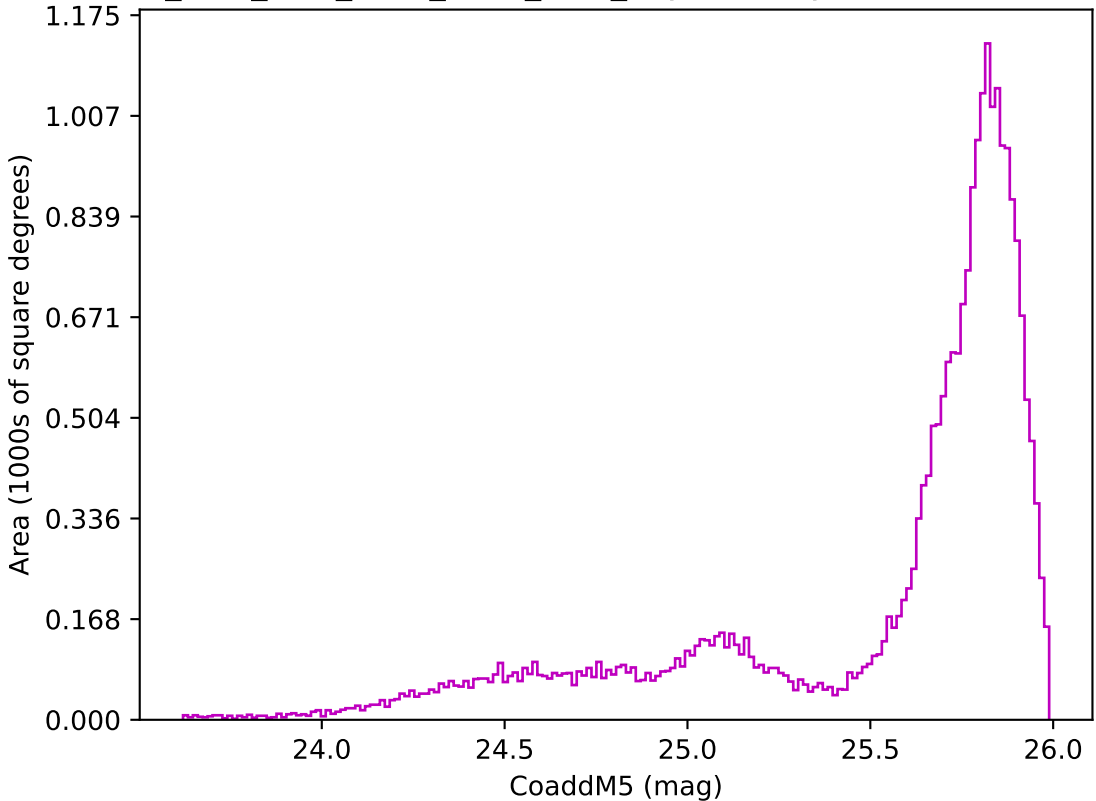
ddf_acor_sf10_lsf30_lsr10_v3.4_10yrs All sky z band: CoaddM5
