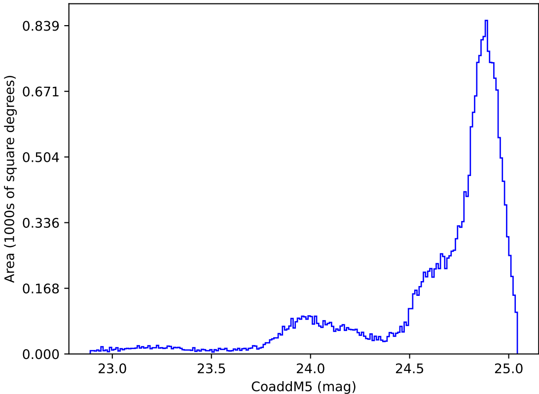
ddf_acor_sf10_lsf30_lsr10_v3.4_10yrs All sky y band: CoaddM5
