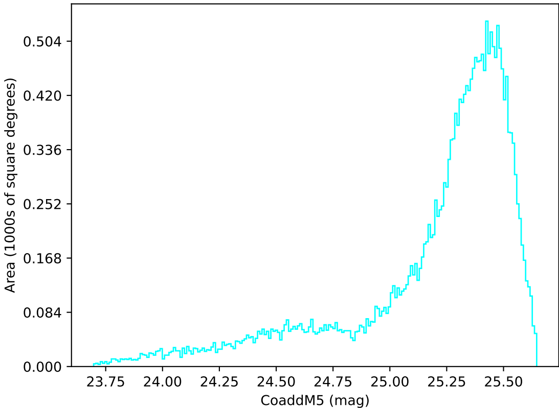
ddf_acor_sf10_lsf30_lsr10_v3.4_10yrs All sky u band: CoaddM5
