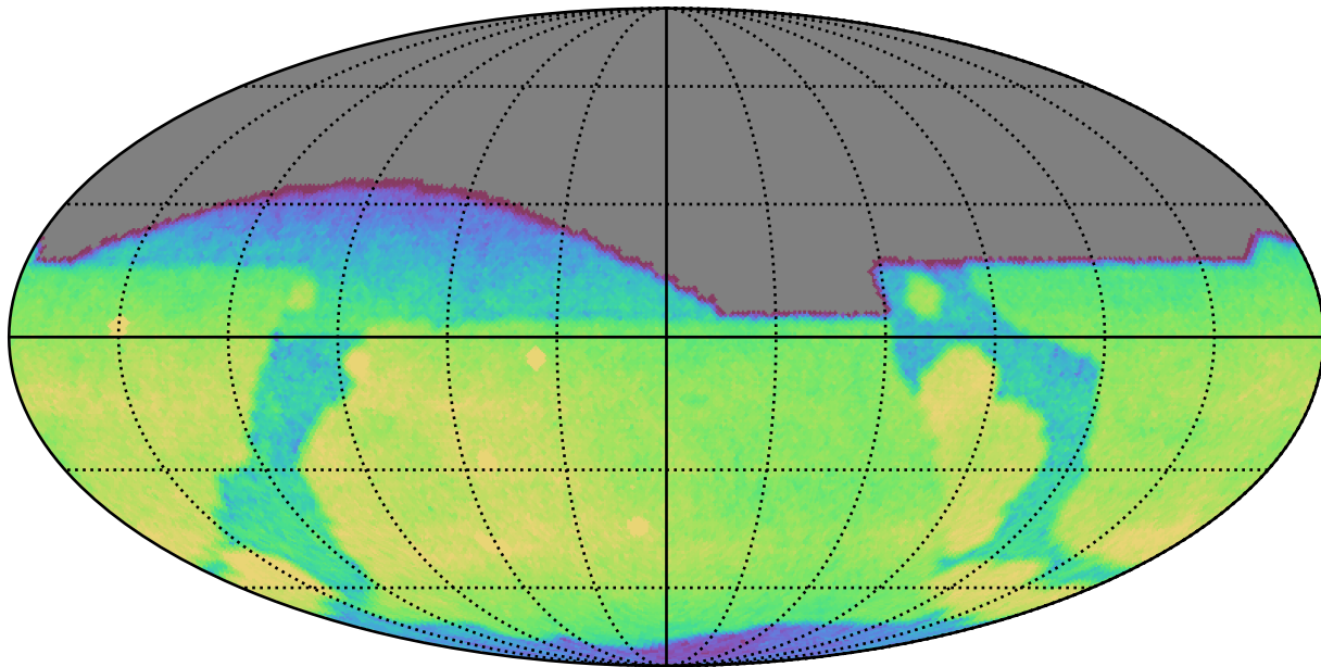
ddf_acor_sf10_lsf30_lsr10_v3.4_10yrs All sky g band: CoaddM5
