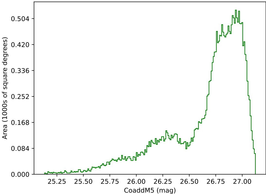
ddf_acor_sf10_lsf30_lsr10_v3.4_10yrs All sky g band: CoaddM5
