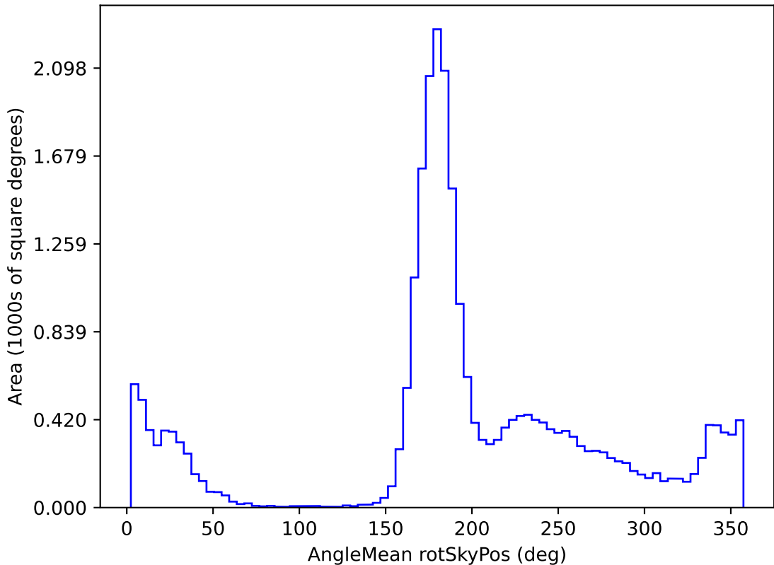
ddf_acor_sf10_lsf30_lsr10_v3.4_10yrs All sky r band: AngleMean rotSkyPos
