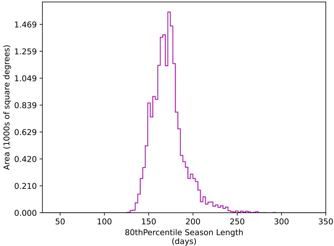
ddf_acor_sf10_lsf30_lsr10_v3.4_10yrs WFD z band: 80thPercentile Season Length
