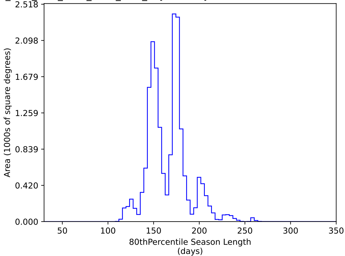
ddf_acor_sf10_lsf30_lsr10_v3.4_10yrs WFD y band: 80thPercentile Season Length
