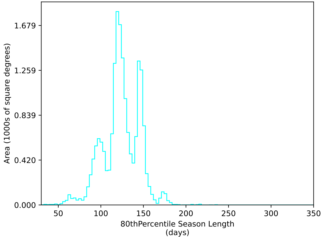
ddf_acor_sf10_lsf30_lsr10_v3.4_10yrs WFD u band: 80thPercentile Season Length
