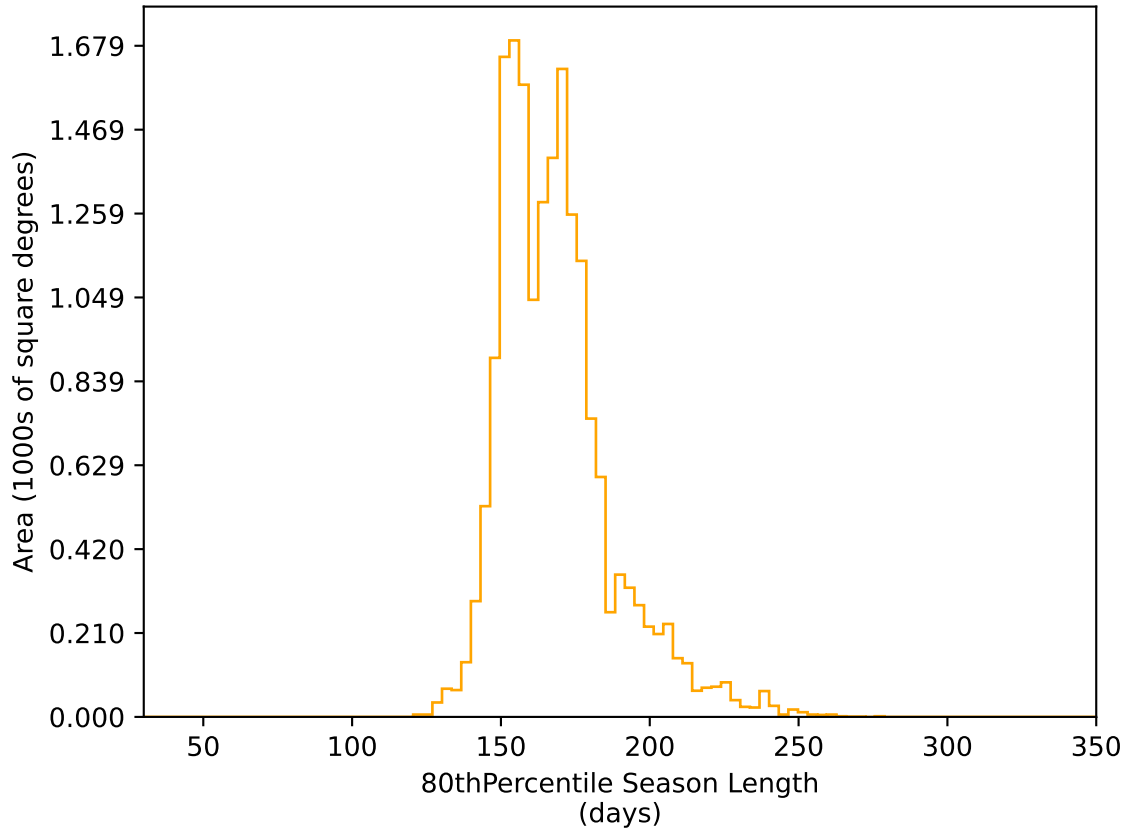
ddf_acor_sf10_lsf30_lsr10_v3.4_10yrs WFD r band: 80thPercentile Season Length
