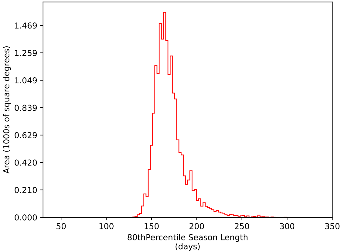
ddf_acor_sf10_lsf30_lsr10_v3.4_10yrs WFD i band: 80thPercentile Season Length
