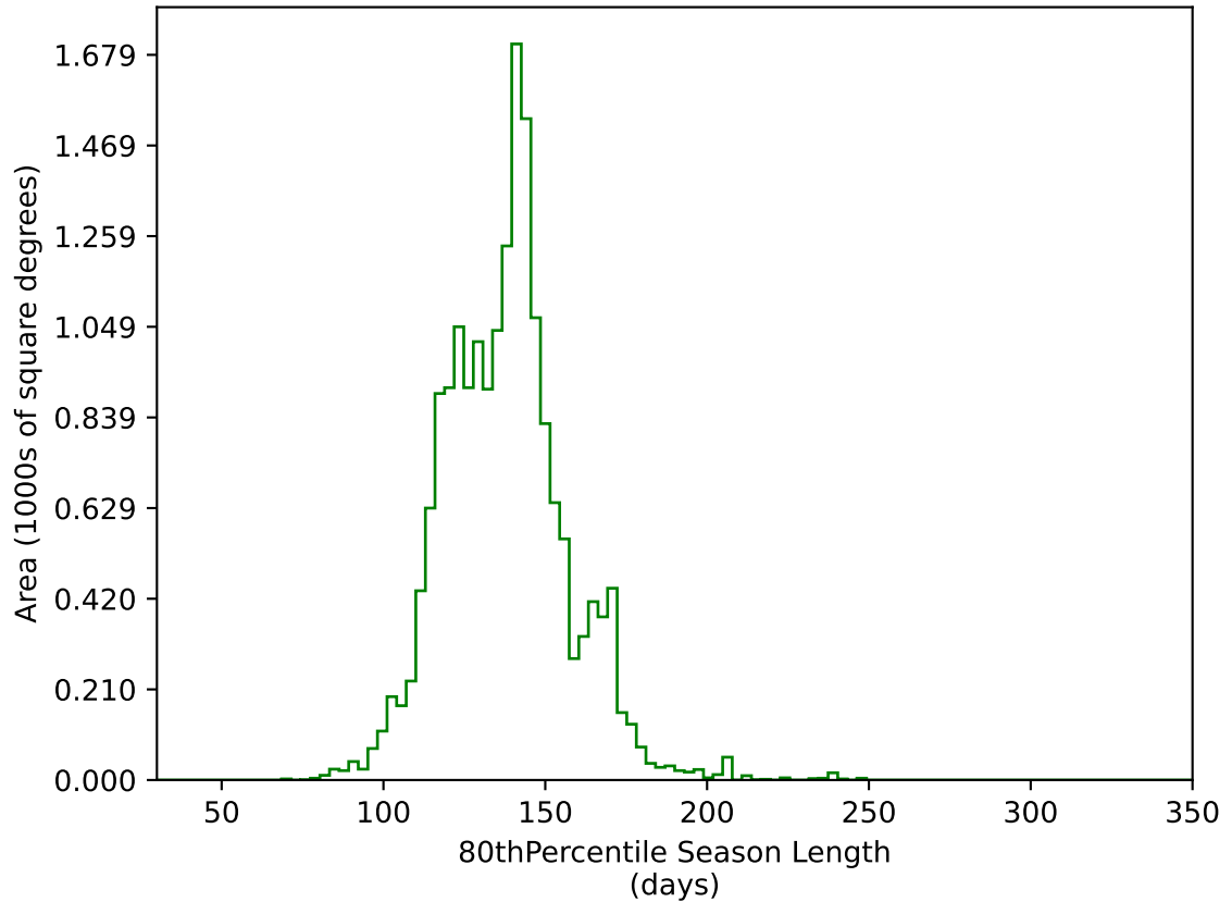
ddf_acor_sf10_lsf30_lsr10_v3.4_10yrs WFD g band: 80thPercentile Season Length
