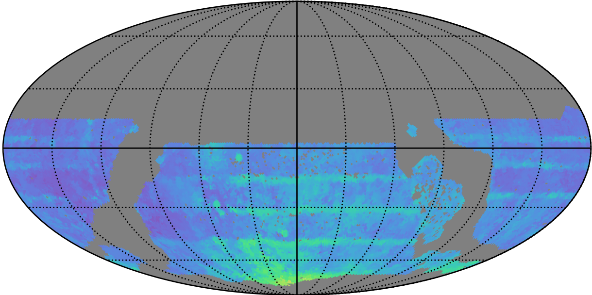
ddf_acor_sf10_lsf30_lsr10_v3.4_10yrs WFD all bands: 80thPercentile Season Length
