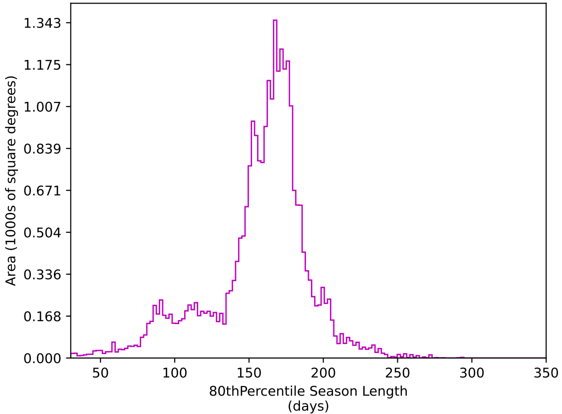
ddf_acor_sf10_lsf30_lsr10_v3.4_10yrs All sky z band: 80thPercentile Season Length
