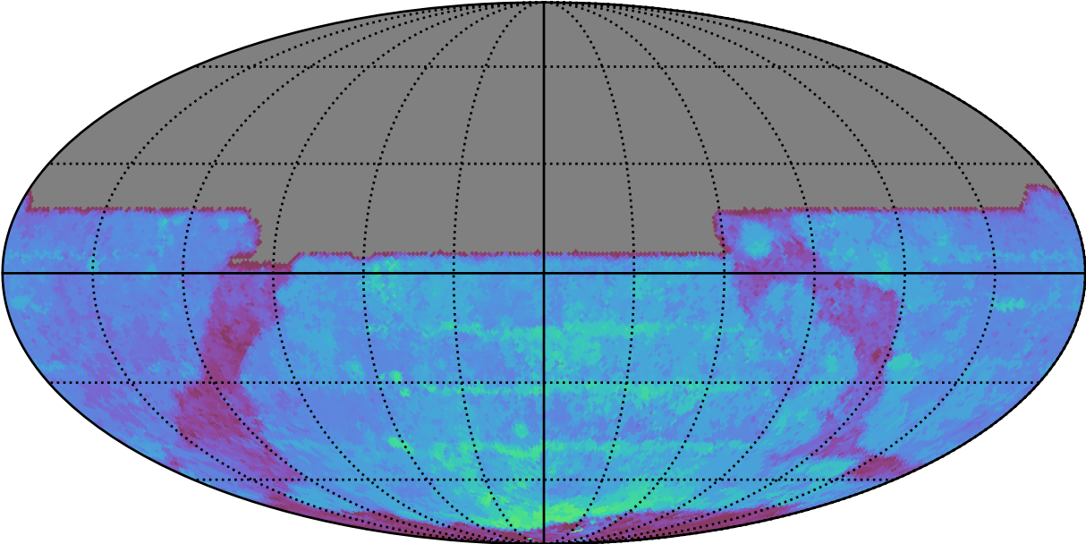
ddf_acor_sf10_lsf30_lsr10_v3.4_10yrs All sky y band: 80thPercentile Season Length
