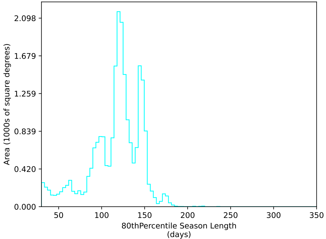
ddf_acor_sf10_lsf30_lsr10_v3.4_10yrs All sky u band: 80thPercentile Season Length
