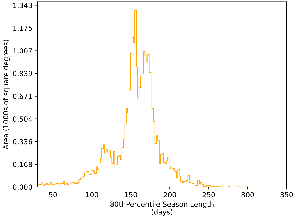
ddf_acor_sf10_lsf30_lsr10_v3.4_10yrs All sky r band: 80thPercentile Season Length
